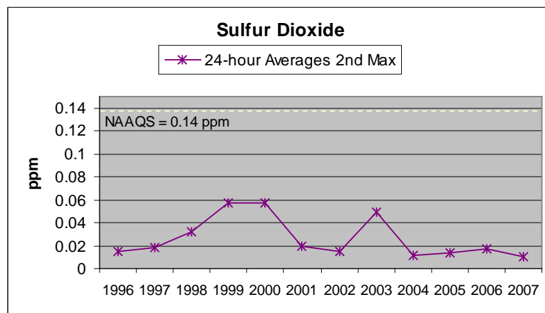
Sulfur Dioxide – Annual Means and 24-Hour / 3-Hour Averages (Ending at 2007 Averaging Period)
