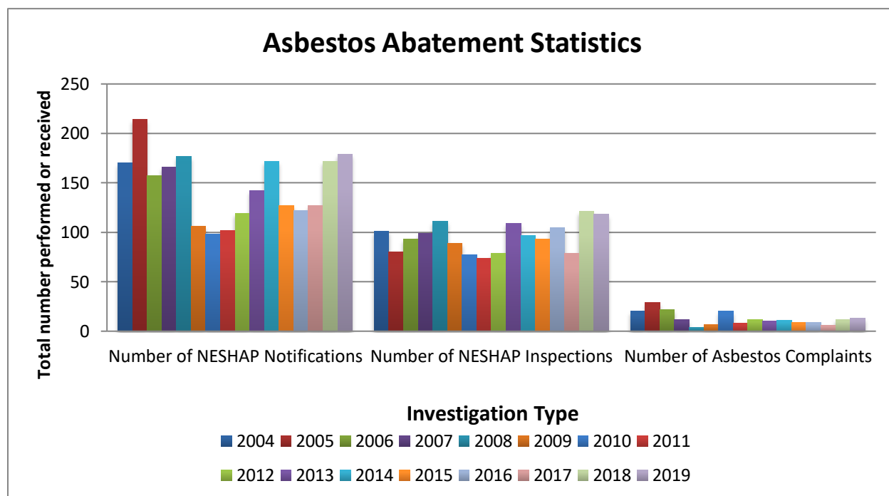
Figure 6.4: The number of NESHAP notifications, NESHAP inspections, and asbestos complaints for 2004-2019.
