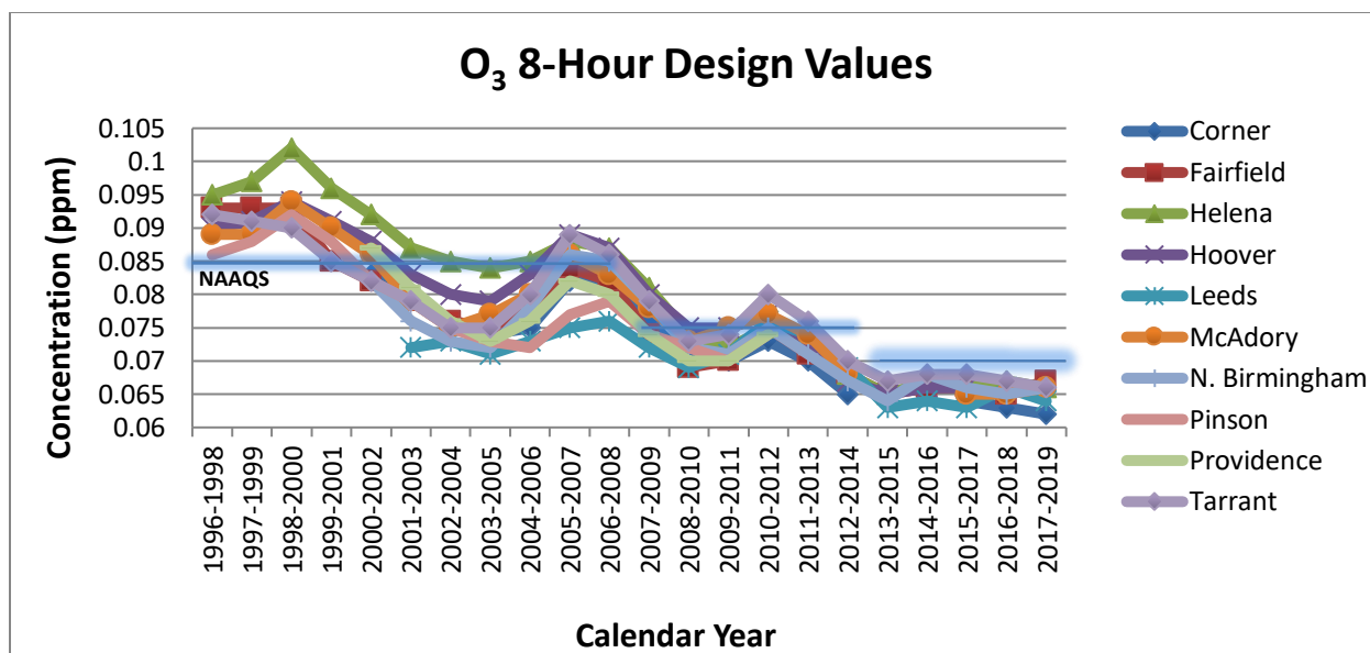
Figure 4.6: 8-hour ozone design values (in ppm) for 1996-2019. The highlighted blue line indicates the NAAQS, which is 0.070 ppm (previously set at 0.085 ppm, in which 0.084 ppm rounded to 0.080 ppm, and at 0.075 ppm).
