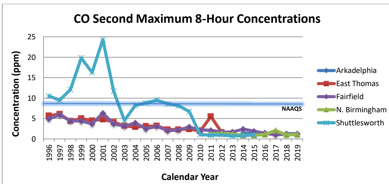
Figure 4.3: Carbon monoxide second maximum 8-hour average concentrations (in ppm) for 1996-2019. The highlighted blue line indicates the NAAQS, which is 9 ppm.
