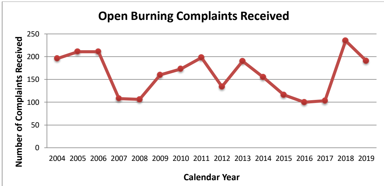
Figure 6.3: The number of open burning complaints received for 2004-2019.
