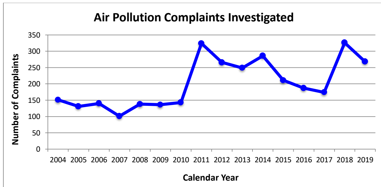
Figure 6.1: The number of air pollution complaints investigated for 2004-2019.
