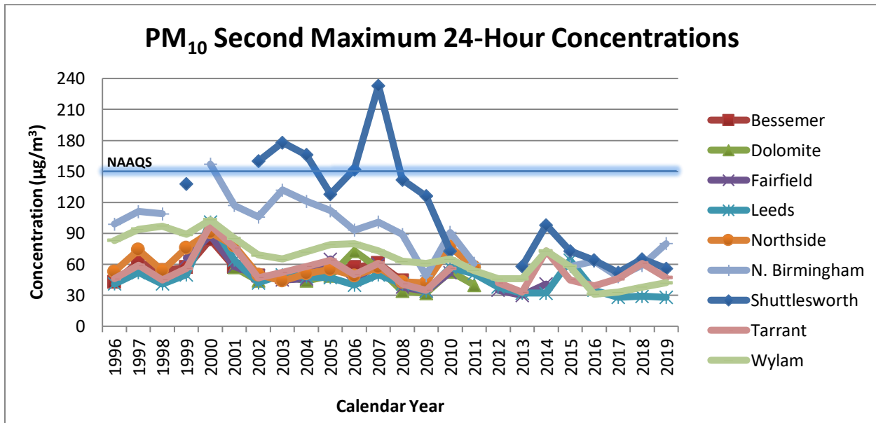
Figure 4.11: The second maximum 24-hour average concentrations of PM 10 for 1996-2019. The highlighted blue line indicates the NAAQS, which is 150 µg/m 3 .
