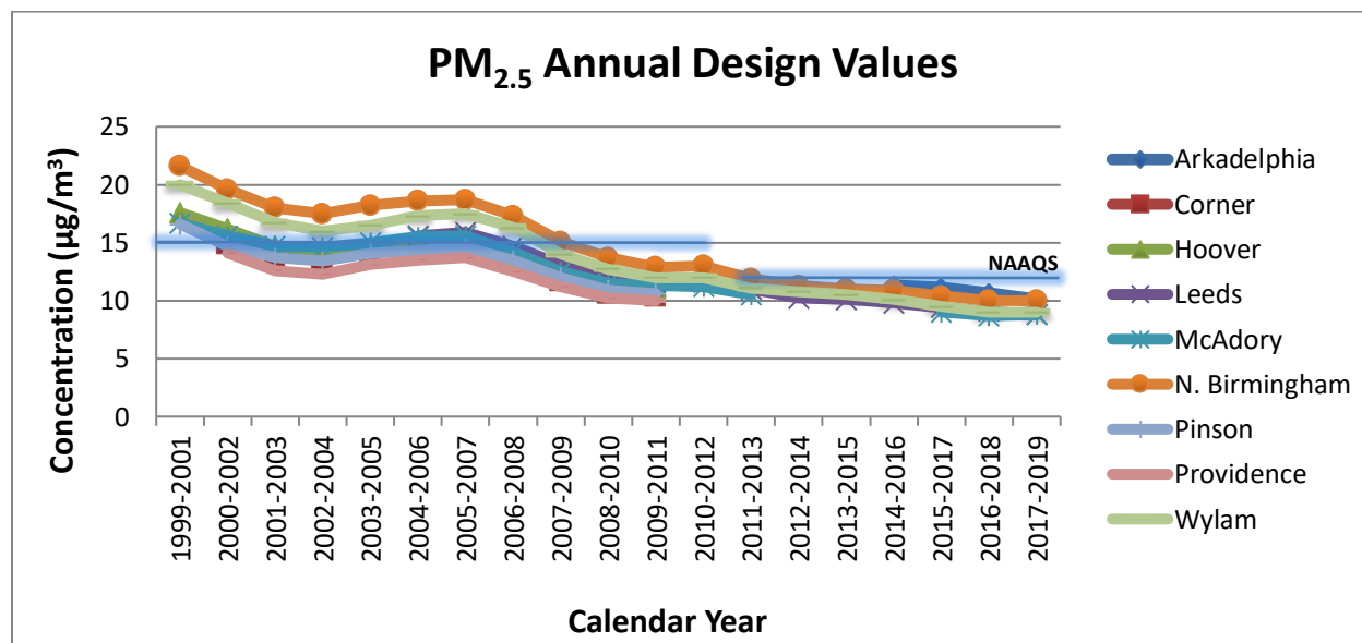
Figure 4.9: Annual PM 2.5 design values (in \mu\text{g}/\text{m}^3 ) for 1999-2019. The highlighted blue line indicates the NAAQS, which is 12 \mu\text{g}/\text{m}^3 (previously set at 15 \mu\text{g}/\text{m}^3 ).
