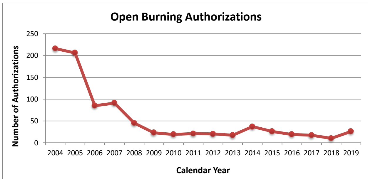
Figure 6.2: The number of open burning authorizations for 2004-2019.
