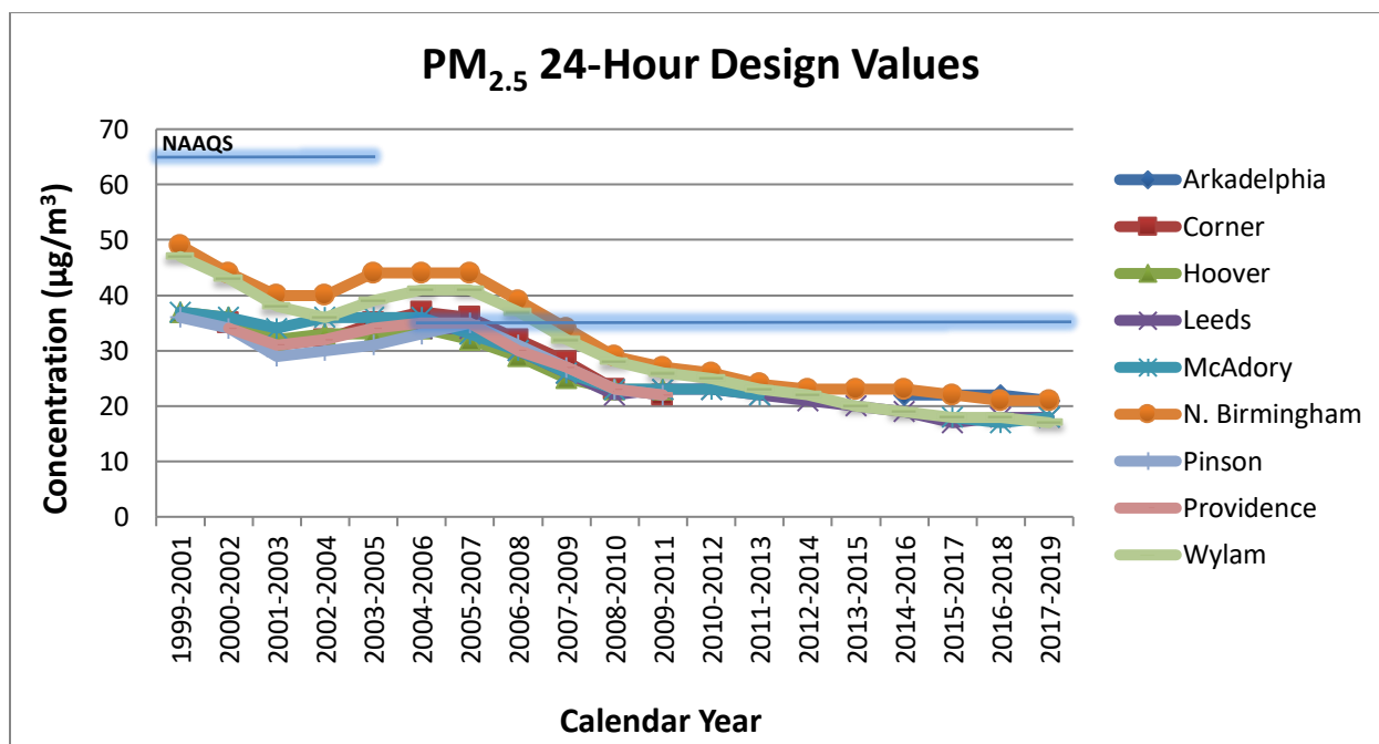
Figure 4.10: 24-hour PM 2.5 design values (in µg/m 3 ) for 1999-2019. The highlighted blue line indicates the NAAQS, which is 35 µg/m 3 (previously set at 65 µg/m 3 ).
