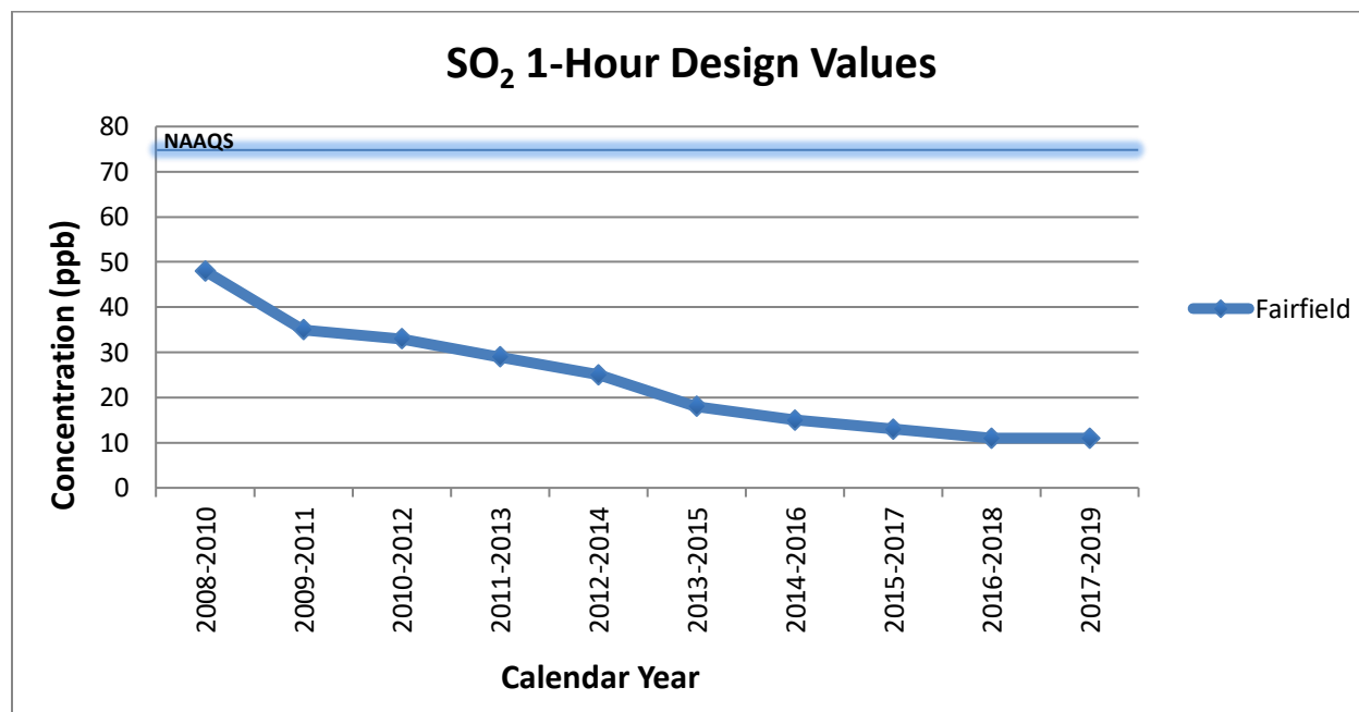
Figure 4.13: 1-hour sulfur dioxide design values (in ppb) for 2008-2019. The highlighted blue line indicates the NAAQS, which is 75 ppb.
