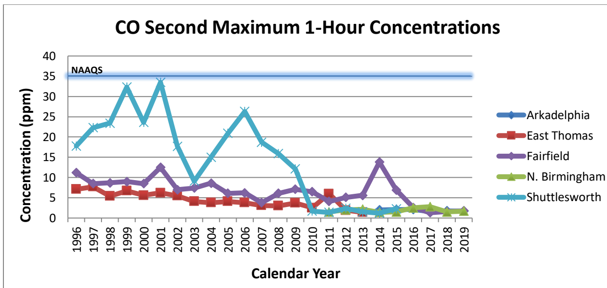
Figure 4.2: Carbon monoxide second maximum 1-hour average concentrations (in ppm) for 1996-2019. The highlighted blue line indicates the NAAQS, which is 35 ppm.
